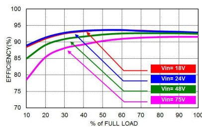
Efficiency vs. Output Load
