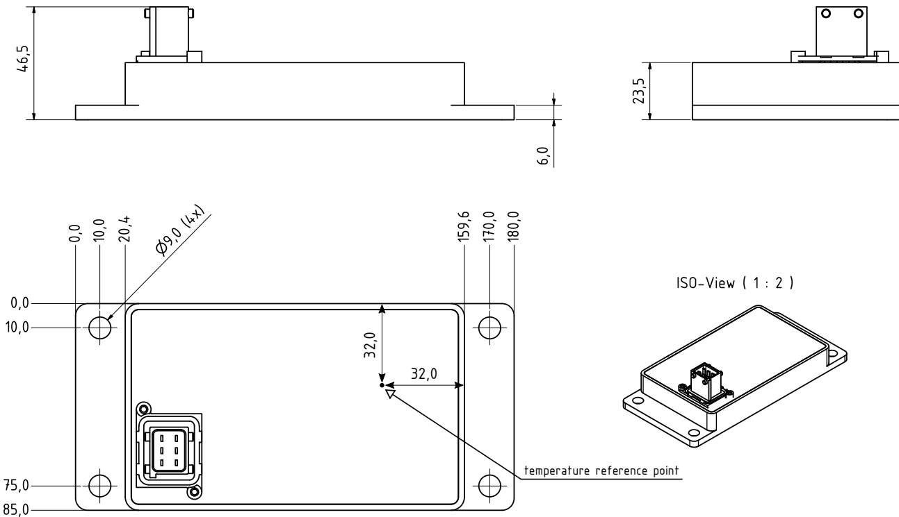
Figure 8.1: Dimensions
