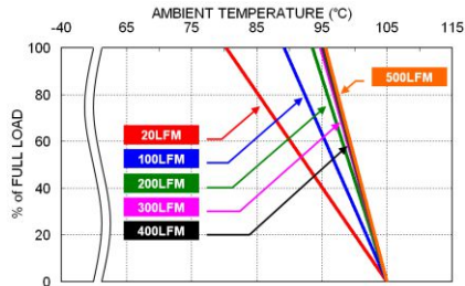
RCD10-48S3P3W Derating Curve
