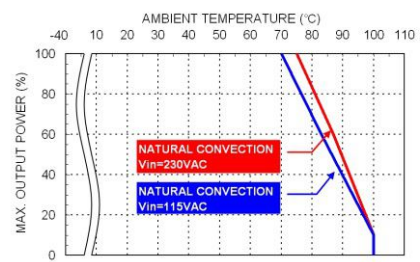
Derating Curve vs. Ambient Temperature MSD30USxxB xx=12/15/24/28/36/48/53 Connector Option : (-M / -T / -D)
