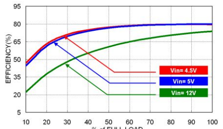
MPS(H)02-05S05 Efficiency vs. Output Current
